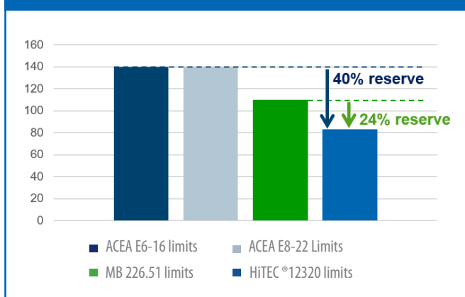
OM 646 LA Cam wear outlet, µm
