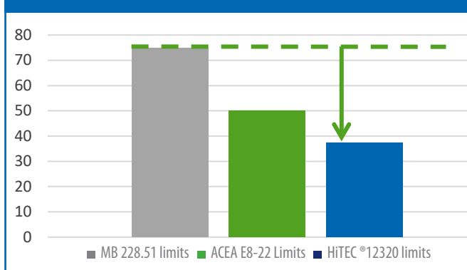
Volvo T-13 Kinematic viscosity increase (40°C), %
