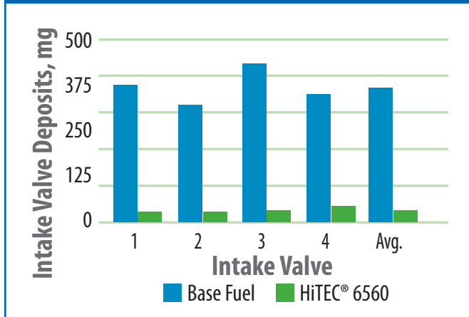
HiTEC® 6560 Keep Clean Performance Ford 2.3L IVD/CCD Test @ 55.1 PTB
