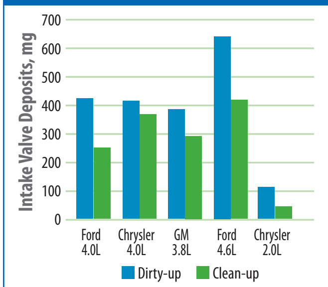
HiTEC® 6560 Clean-up Performance Fleet Test @ 78 PTB
